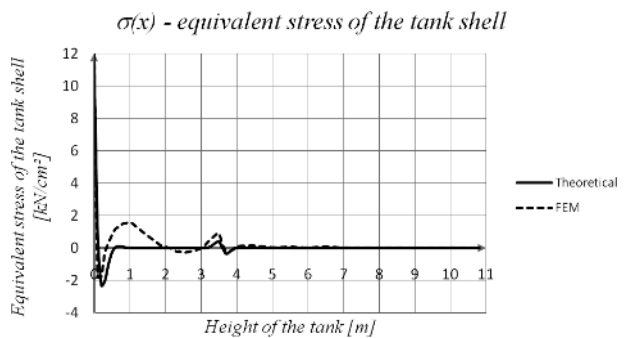
Figure 12. Diagram of distribution of equivalent stress of the tank shell obtained by the application of FEM
