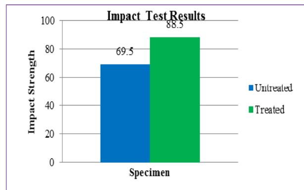
Figure 9: Impact Strength of untreated and treated fiber reinforced composite
