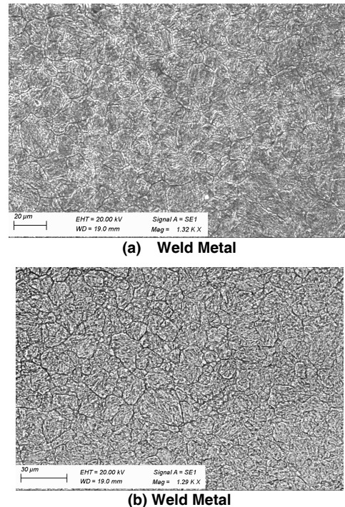
Figure: 9 SEM image Argon 50% & Helium 50% weld Specimen
