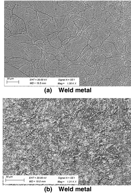
Figure 8: SEM image Helium weld Specimen
