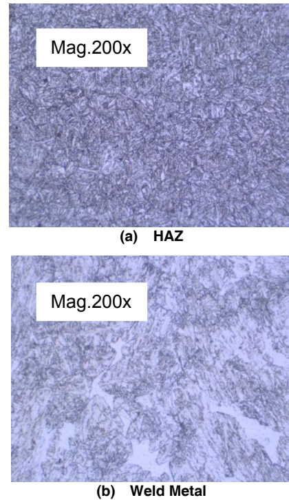
Figure 5: Microstructure of Helium gas specimen HAZ & WM
