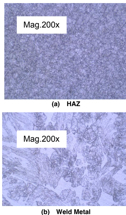
Figure 4: Microstructure of Argon gas specimen HAZ & WM
