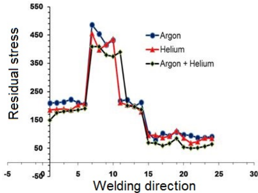
Figure 3: Residual stress comparisons
