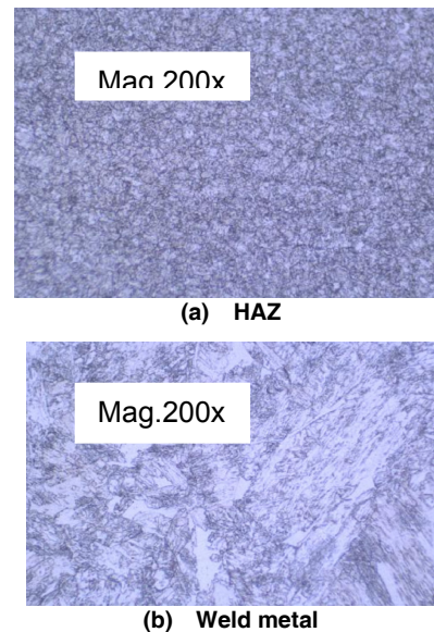
Figure 6: Microstructure image of Argon 50% & Helium 50% gas specimen HAZ and WM
