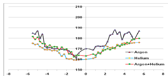
Figure 2: Micro hardness for different shielding gas
