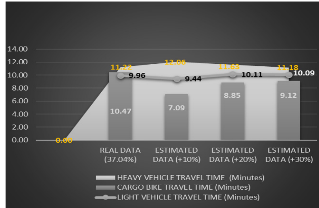
Figure-13: Estimation Of Vehicle Travel Time, Within City Limits By Increasing Cargo Bike Count In Roads
