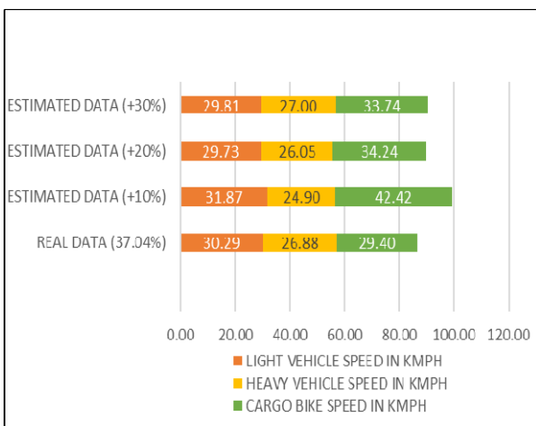
Figure-12: Estimation Of Vehicle Travel Speed, Within City Limits For Conditional Variables
