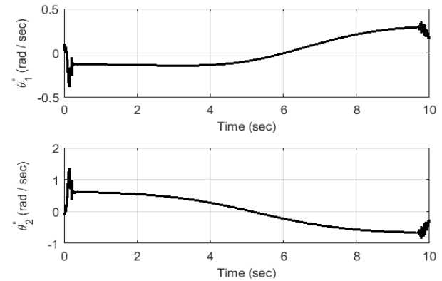
Figure 8. The angular velocity with the kinematic NMPC-PSO
