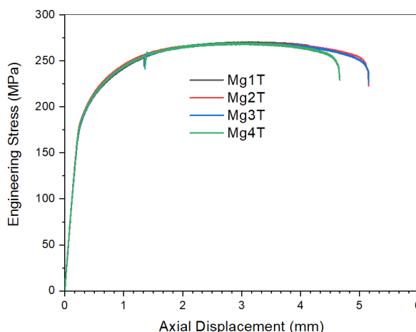
Figure 5. The relationship between the stress incremental and the change in specimen length
