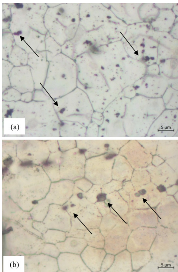
Figure 3. Original microstructure of Mg AZ31B in extrusion condition in (a) Transversal and (b) Longitudinal directions
