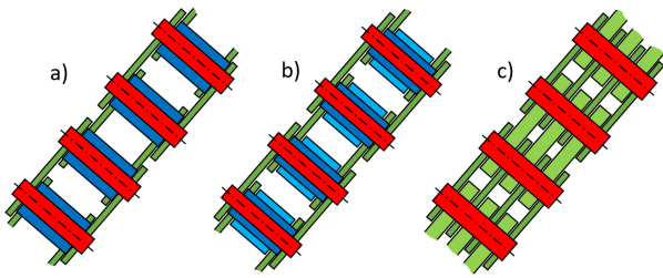
Figure 1. Timing chain types: a) bush chain, b) roller chain, c) toothed chain (silent chain)
