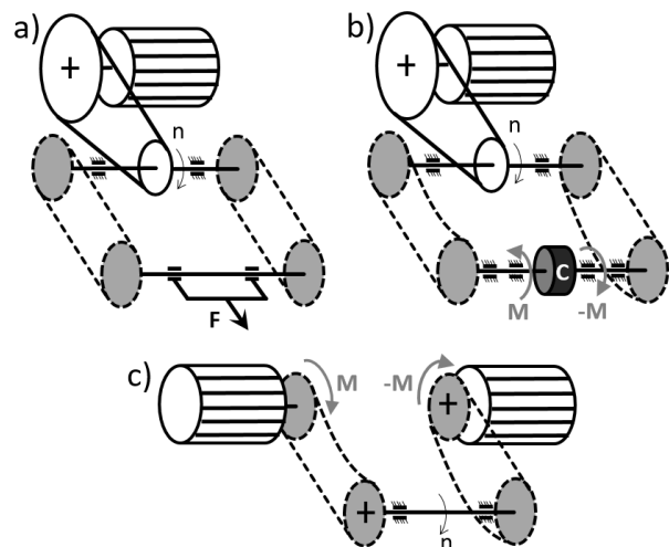
Figure 4. Tensioning methods on-chain test benches
