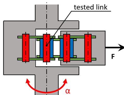
Figure 6. Schematic setup of chain joint tribometer
