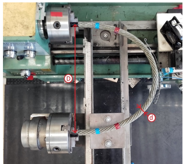
Figure 2. Experimental apparatus used for testing ropes
