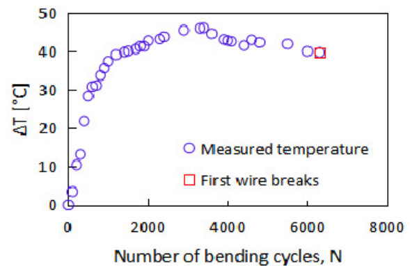
Figure 4. The trend of rope temperature during a rotary bending fatigue test
