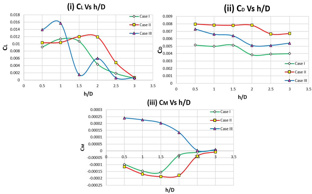
Figure 5: Trends of the aerodynamic coefficients like lift, drag, and moment are depicted for all the h/D ratios taken for the comparative analysis.
