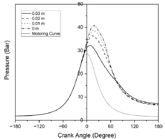
Figure 6. Pressure (Pa) vs. crank angle (degree) for different positions of the spark plug in the single-spark engine.
