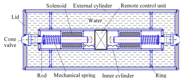
Figure 3. Longitudinal section of the bathometer (See also A–A Figure 2)
