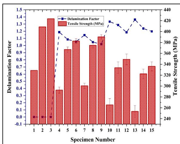
Figure 23. Comparison of residual Tensile strength for various specimens.
