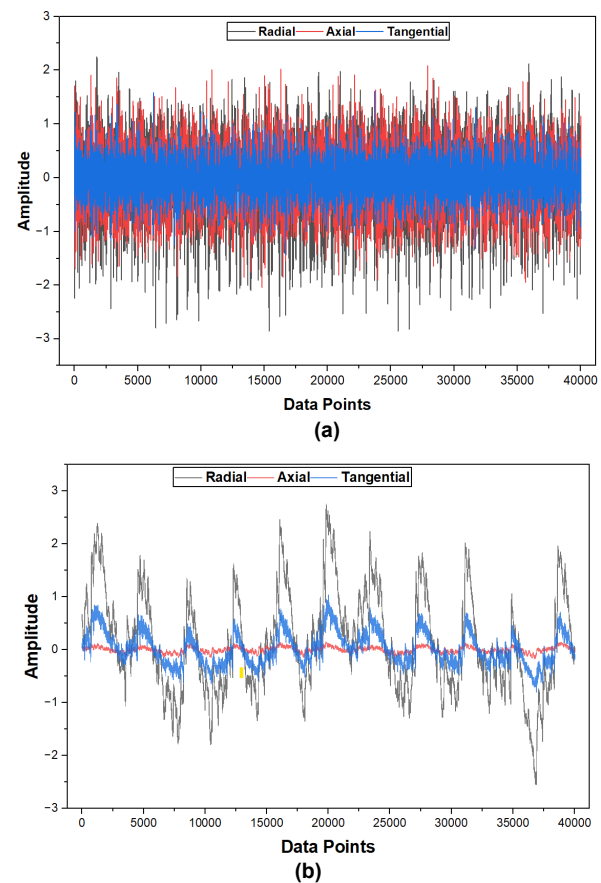
Figure 1. Acquired Vibration Signal (a) Normal Bearing (b) Bearing with cage defect
