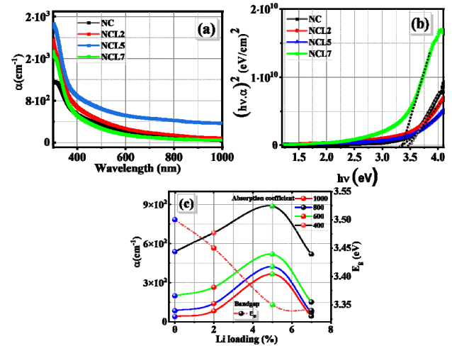
Figure 6. (a) Absorption coefficient, (b) Tauc's plot, and (c) absorption coefficient with Li content of \text{Li}_x\text{Cu}_{0.05}\text{Ni}_{0.95-x}\text{O} films
