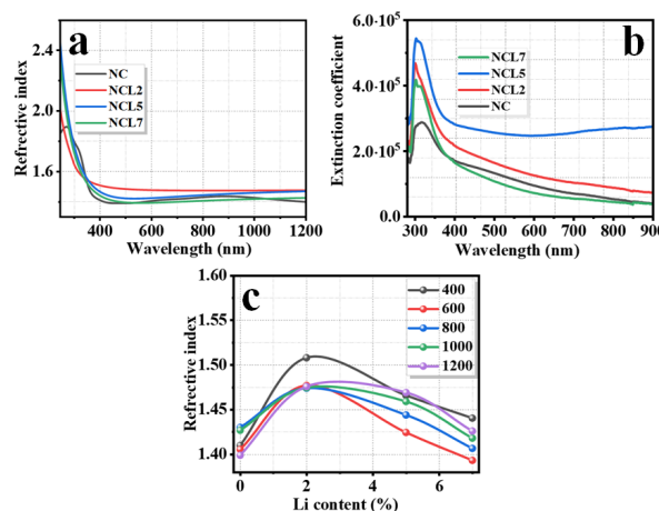
Figure 9. (a) Refractive index vs. wavelength, (b) Extinction coefficient vs. wavelength, and (c) refractive index with Li content of \text{Li}_x\text{Cu}_{0.05}\text{Ni}_{0.95-x}\text{O} films.
