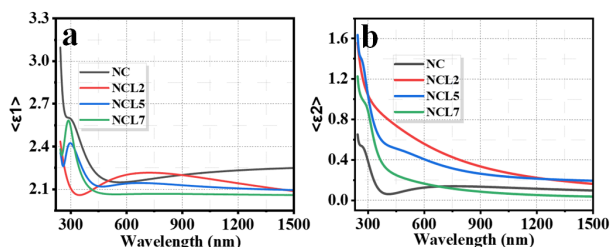
Figure 7. (a) Epsilon ( \epsilon_1 ) and (b) Epsilon ( \epsilon_2 ) of \text{Li}_x\text{Cu}_{0.05}\text{Ni}_{0.95-x}\text{O} films
