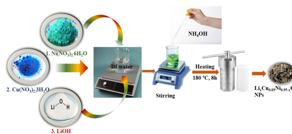
Figure 1. Schematic diagram for the synthesis process of Li x Cu 0.05 Ni 0.95–x O
