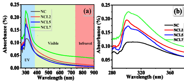
Figure 5. Absorbance value of the dispersion solution of \text{Li}_x\text{Cu}_{0.05}\text{Ni}_{0.95-x}\text{O} NPs in (a) wide range and (b) short range
