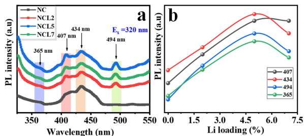
Figure 10. (a) Photoluminescence (PL) and (b) PL with Li content
