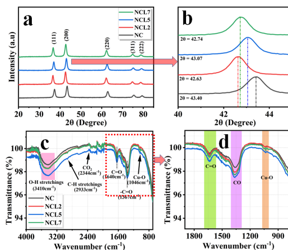
Figure 2. (a, b) X-ray diffraction patterns and (c, d) FTIR Fourier-transform infrared transmission spectra of \text{Li}_x\text{Cu}_{0.05}\text{Ni}_{0.95-x}\text{O}
