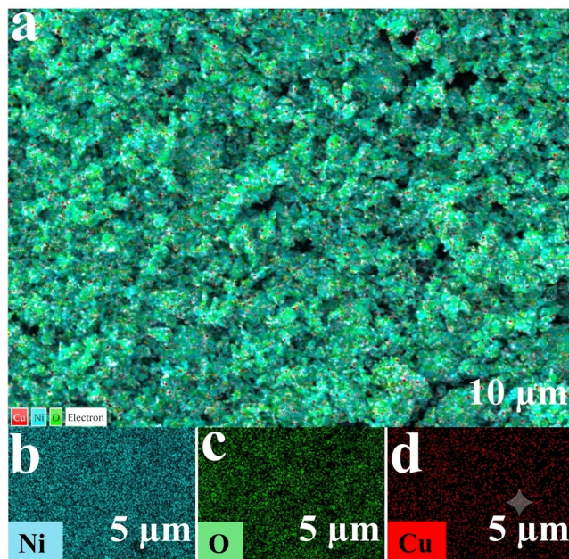
Figure 4. Energy dispersive X-ray spectroscopy of \text{Li}_x\text{Cu}_{0.05}\text{Ni}_{0.95-x}\text{O} for x = 2\% for (a) Mix, (b) Ni, (c) O, and (d) Cu
