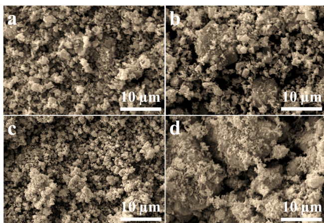
Figure 3. Scanning electron microscopy images of \text{Li}_x\text{Cu}_{0.05}\text{Ni}_{0.95-x}\text{O} for (a) x = 0\% , (b) x = 2\% , (c) x = 5\% , and (d) x = 7\%
