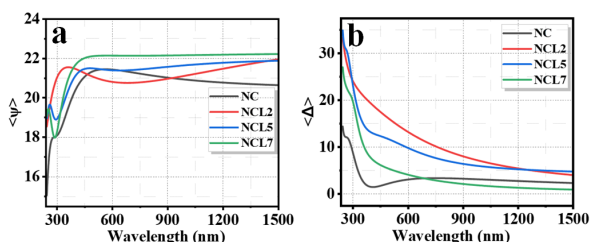
Figure 8. (a) Psi ( \psi ) ;(b) Delta ( \Delta ) of \text{Li}_x\text{Cu}_{0.05}\text{Ni}_{0.95-x}\text{O} films
