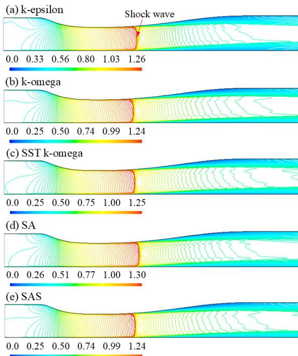
Figure 7. Differences in the behavior of the Mach number flow field for r_p = 0.82
