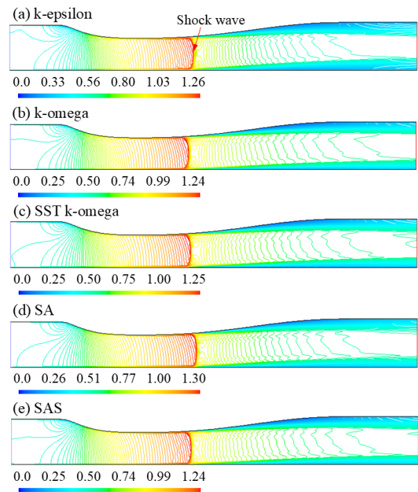
Figure 9. Differences in the behavior of the Mach number flow field for r_p = 0.72
