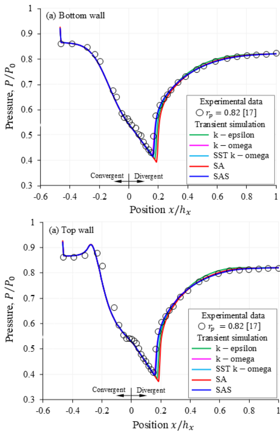
Figure 3. Comparison of curves from five turbulence models with experimental pressure data for r_p = 0.82 [17]
