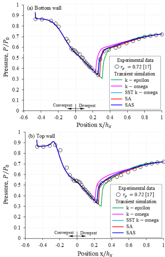
Figure 4. Comparison of curves from five turbulence models with experimental pressure data for r_p = 0.72 [17]
