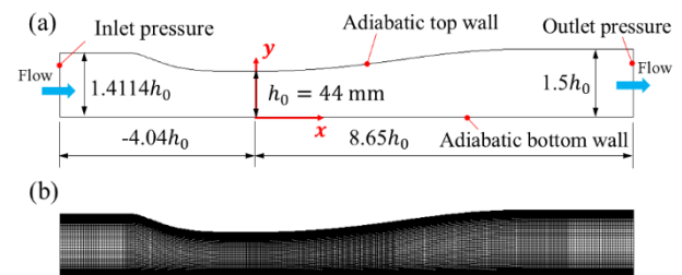
Figure 1. (a) 2D computational domain for the transonic diffuser geometry. (b) Meshed domain with structured quadrilateral cells: Mesh 3 with 46970 elements
