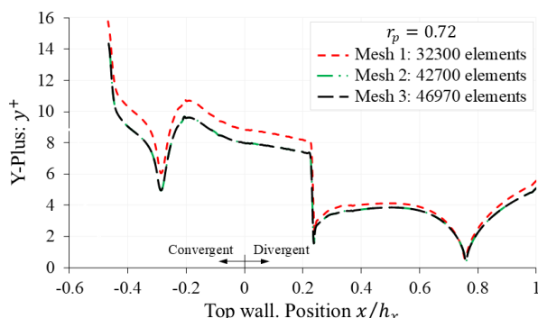
Figure 2. y^+ behavior for the meshed domain: Mesh 1, Mesh 2, and Mesh 3
