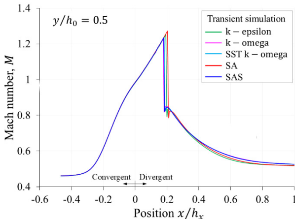
Figure 8. Mach number curves evaluated for five turbulence models for r_p = 0.82
