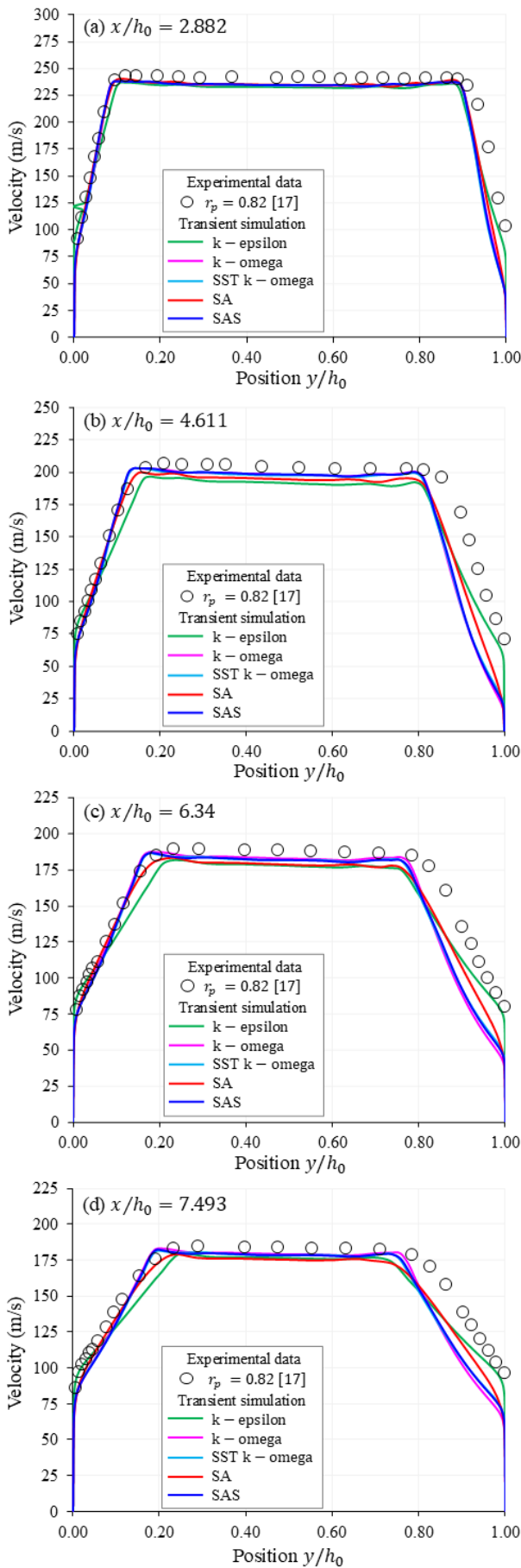
Figure 5. Comparison of curves from five turbulence models with experimental velocity data for r_p = 0.82 [17]
