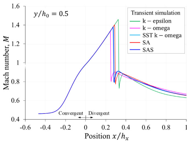
Figure 10. Mach number curves evaluated for five turbulence models for r_p = 0.72
