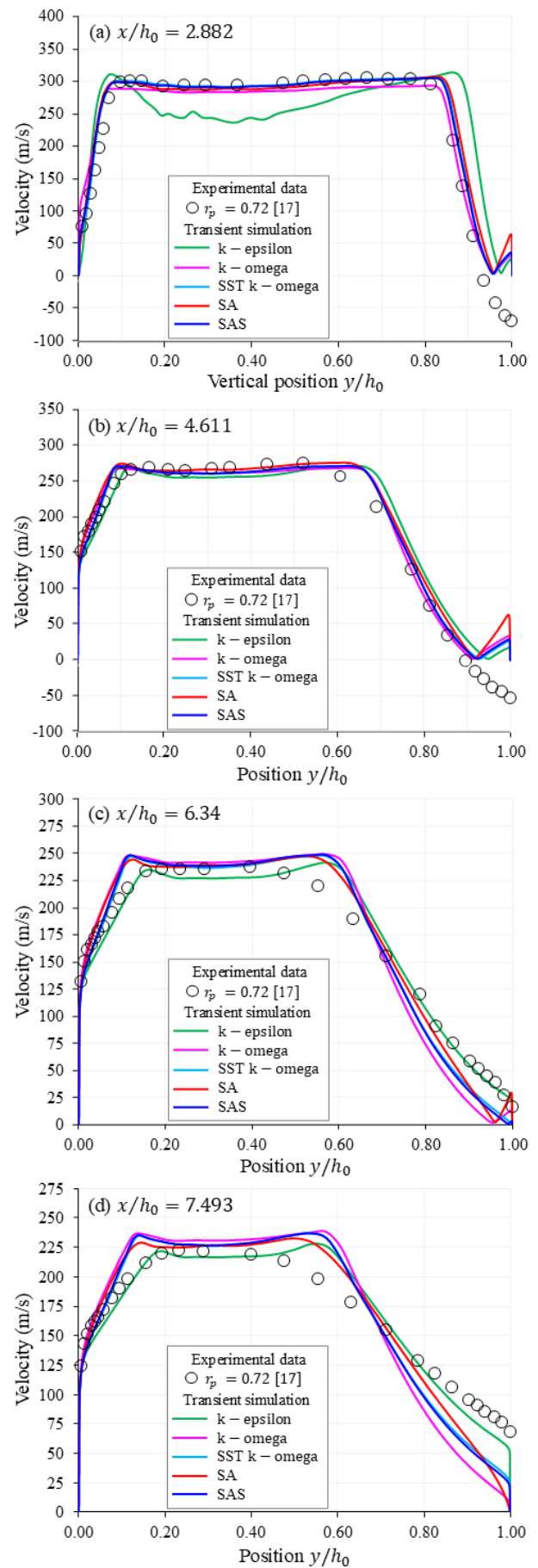
Figure 6. Comparison of curves from five turbulence models with experimental velocity data for r_p = 0.72 [17]
