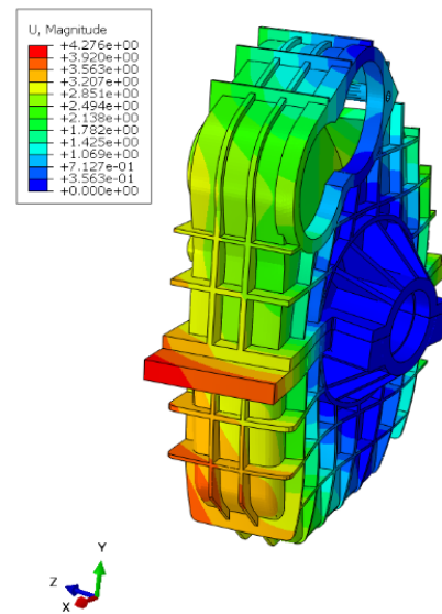
Figure 5. Second-order mode shape
