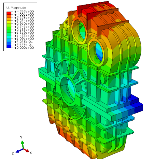
Figure 25. First-order mode shape of the optimized housing
