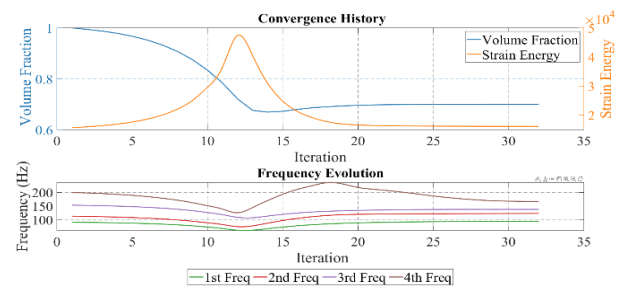
Figure 10. Iteration process with compliance as the optimization objective
