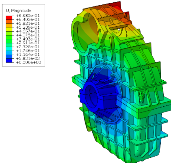
Figure 24. Displacement contour of the optimized housing (2)
