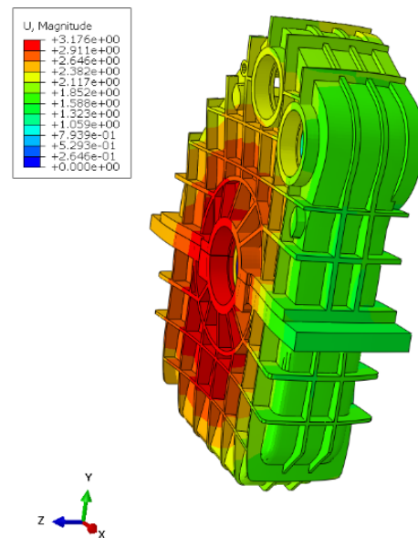
Figure 6. Third-order mode shape
