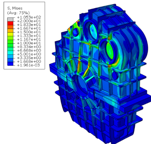
Figure 21. Stress contour of the optimized housing (1)
