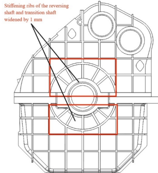
Figure 20. Model modification diagram (2)
