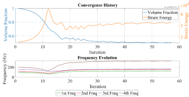
Figure 14. Iteration process with the fourth-order frequency as the optimization objective
