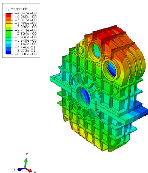
Figure 4. First-order mode shape
