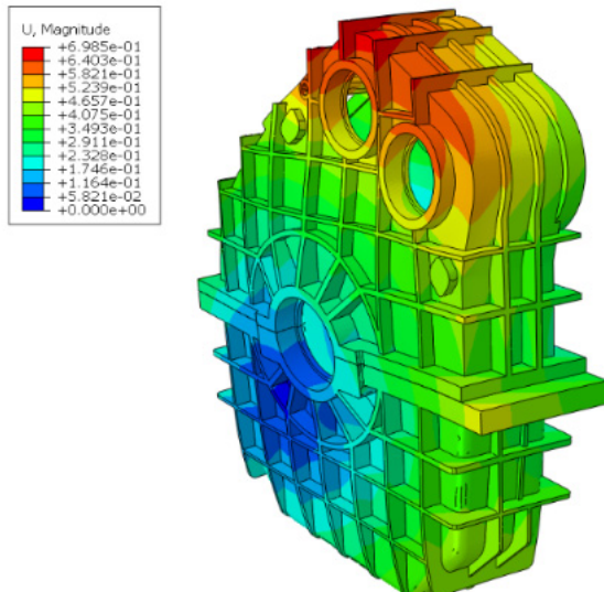
Figure 23. Displacement contour of the optimized housing (1)
