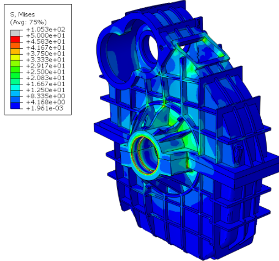
Figure 22. Stress contour of the optimized housing (2)
