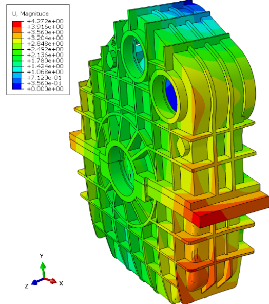
Figure 26. Second-order mode shape of the optimized housing
