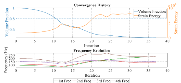
Figure 11. Iteration process with the first-order frequency as the optimization objective
