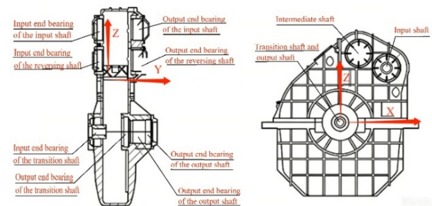
Figure 1. Force diagram of the housing
