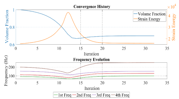
Figure 16. Iteration process with entropy weight objective weights
