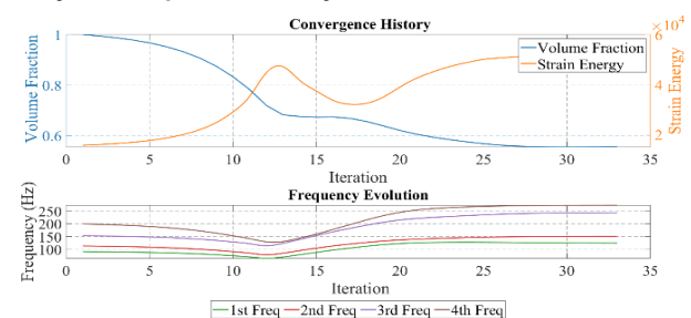
Figure 13. Iteration process with the third-order frequency as the optimization objective
