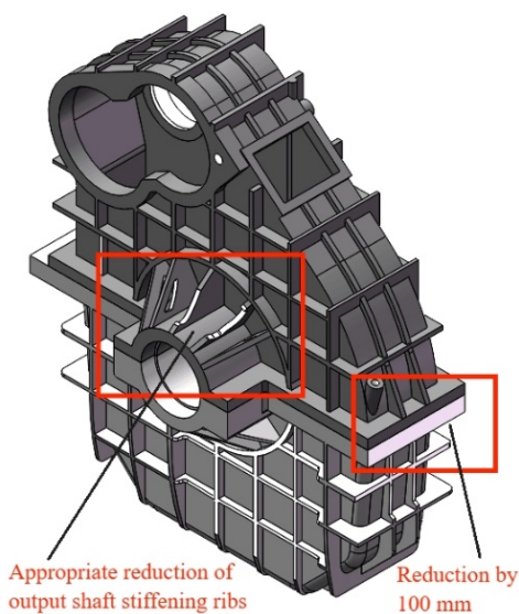
Figure 19. Model modification diagram (1)
