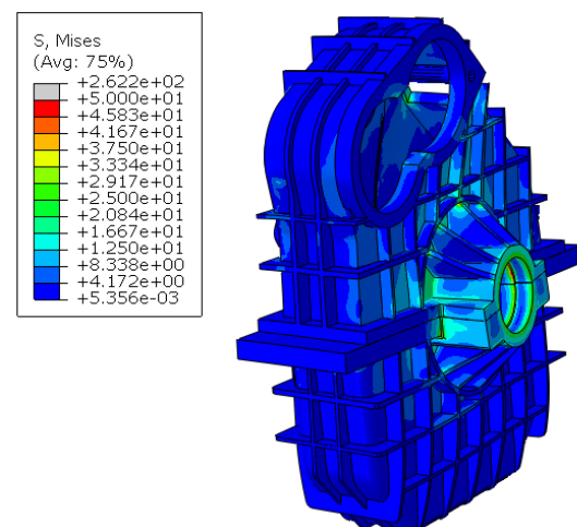
Figure 2. Stress contour of the housing
