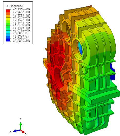
Figure 27. Third-order mode shape of the optimized housing
