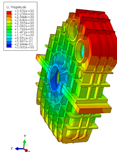
Figure 7. Fourth-order mode shape
