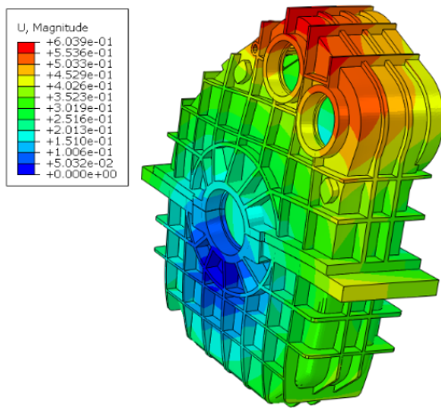
Figure 3. Displacement contour of the housing
