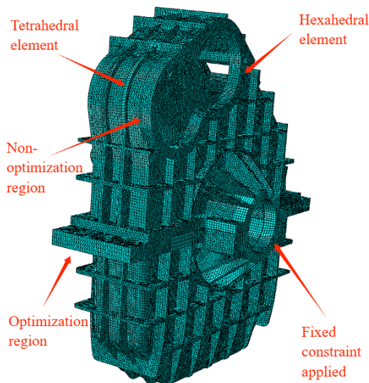
Figure 8. Finite element model diagram
