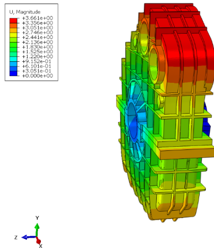
Figure 28. Fourth-order mode shape of the optimized housing
