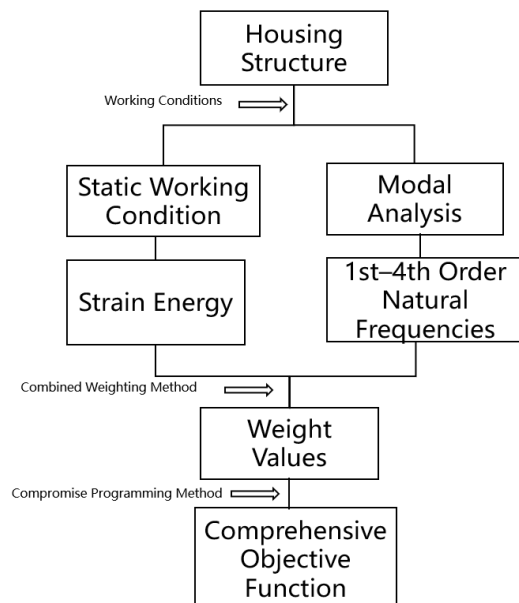
Figure 9. Optimization flow chart
