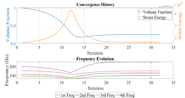
Figure 17. Iteration process with combined weights
