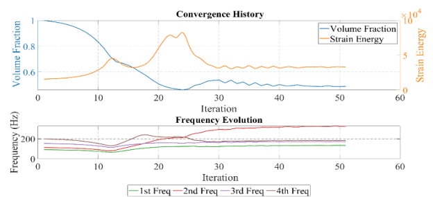
Figure 12. Iteration process with the second-order frequency as the optimization objective
