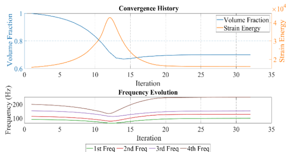
Figure 15. Iteration process with AHP subjective weights
