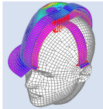
Figure 2. Figure 2: Macro-scale structural Finite Element Analysis (FEA) grid setup of the industrial hard hat assembly, displaying the doubly curved shell element discretization of the outer protective helmet shell coupled with the discrete strap modeling of the underlying internal skull suspension network.
