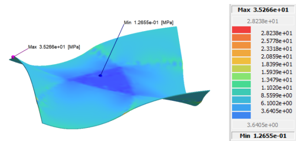
Figure 10. Von Mises stress distribution for configuration C3, t = 1 mm
