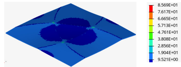
Figure 16. Von Mises stress distribution for configuration C3, t = 2 mm
