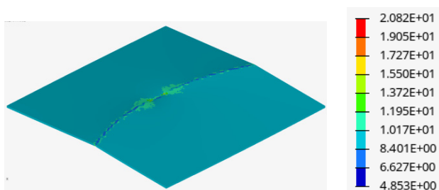
Figure 14. Von Mises stress distribution for configuration C1, t = 2 mm
