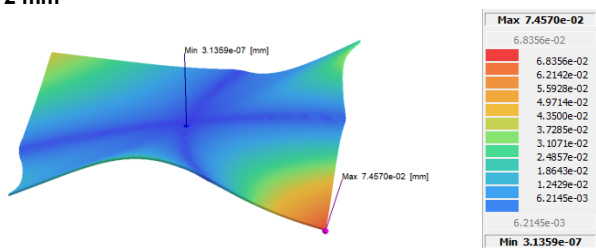
Figure 6. Displacement distribution for configuration C2, t = 1.5 mm
