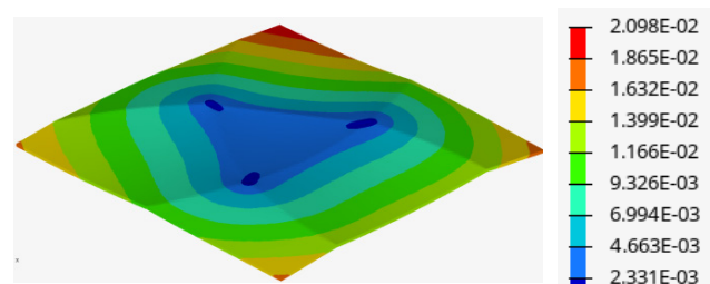
Figure 13. Displacement distribution for configuration C3, t = 2 mm
