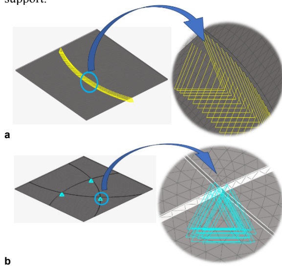
Figure 3. Boundary condition strategies:(a) fully constrained curved folding path; (b) distributed multi-node constraints.
