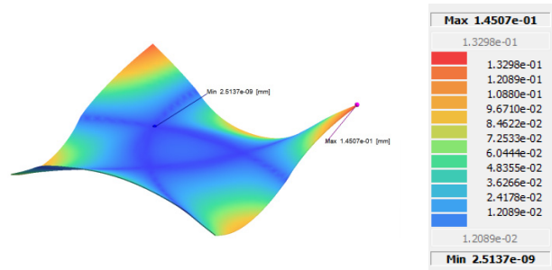
Figure 7. Displacement distribution for configuration C3, t = 1 mm
