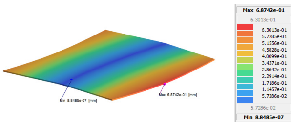
Figure 5. Displacement distribution for configuration C1, t = 2 mm
