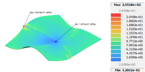
Figure 9. Von Mises stress distribution for configuration C2, t = 0.7 mm
