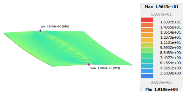
Figure 8. Von Mises stress distribution for configuration C1, t = 0.7 mm
