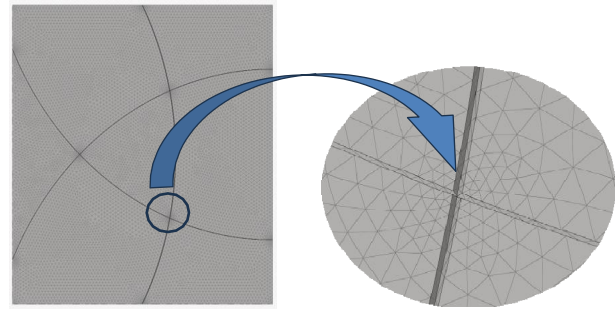
Figure 4. Curvature-based mesh refinement in the intersection region of curved folding paths
