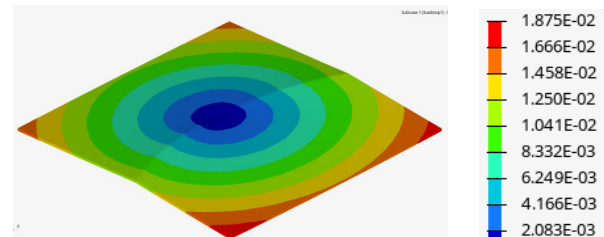
Figure 11. Displacement distribution for configuration C1, t = 2 mm
