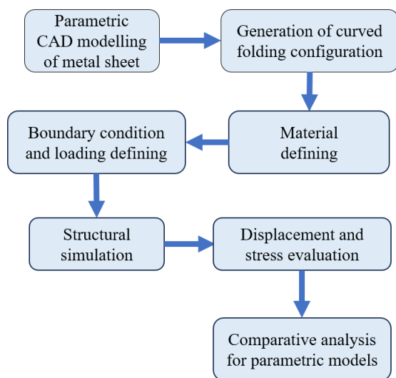
Figure 1. Numerical investigation workflow
