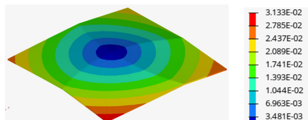
Figure 12. Displacement distribution for configuration C2, t = 2 mm
