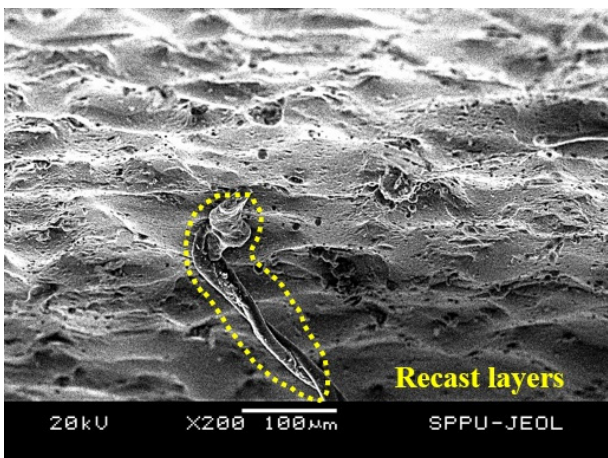
Figure 19. Recast layer formation with nanodielectric
