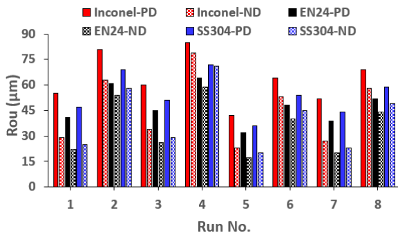
Figure 13. Roundness error varying with cutting conditions for different materials
