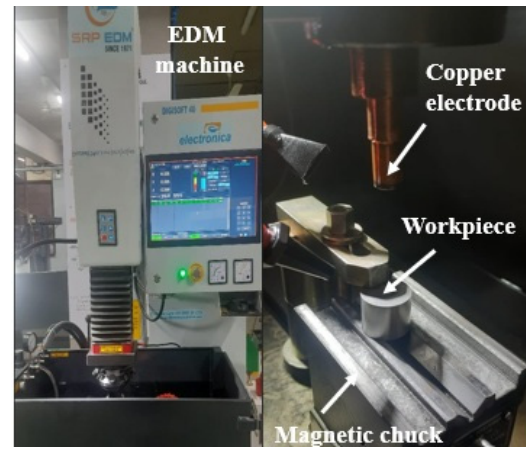
Figure 7. Experimental setup
