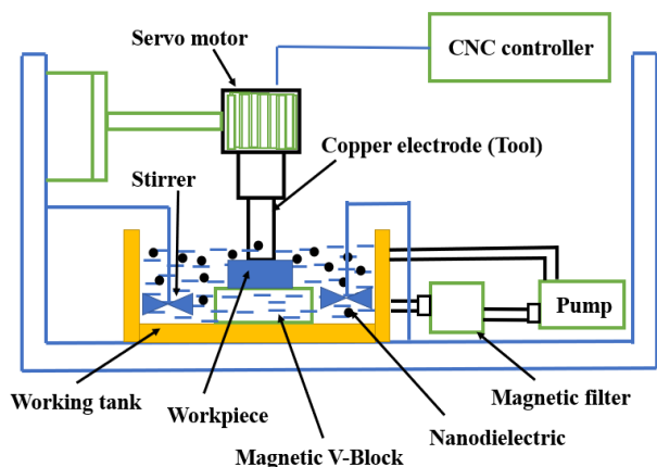
Figure 1. EDM drilling setup
