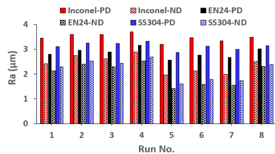
Figure 12. Surface roughness varying with cutting conditions for different materials
