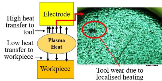
Figure 10. Tool wear due to localised heating
