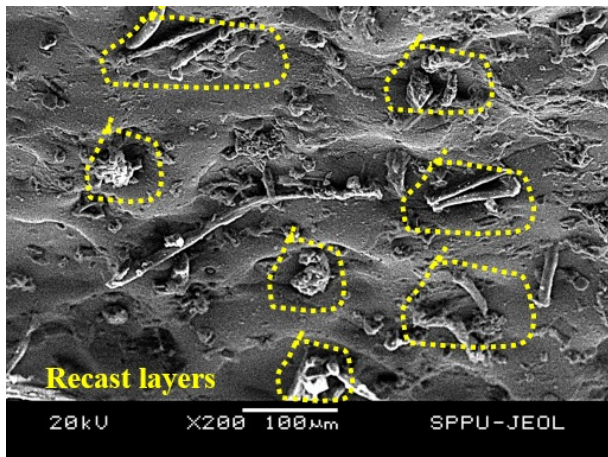
Figure 18. Recast layer formation with plain dielectric
