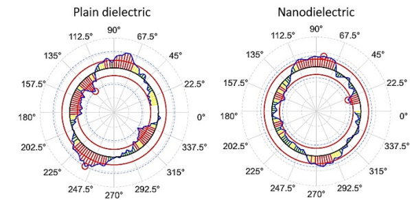
Figure 15. Polar plots for roundness: SS304
