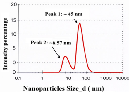
Figure 4. DLS analysis of Graphene nanodielectric
