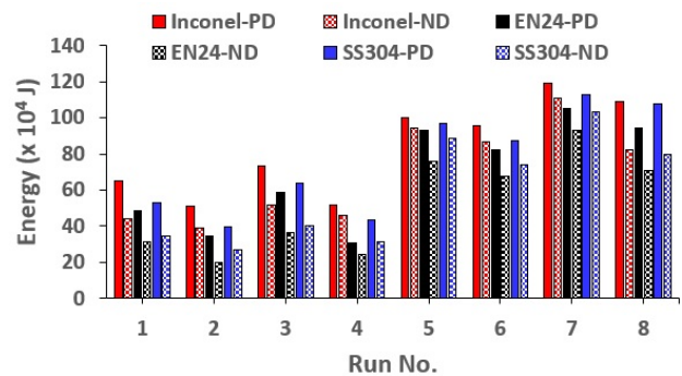
Figure 20. Energy consumption varying with cutting conditions for different materials
