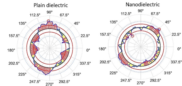
Figure 16. Polar plots for roundness: EN24
