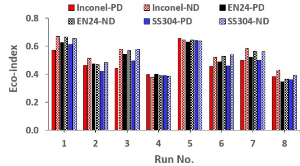
Figure 21. Eco-index varying with cutting conditions for different materials
