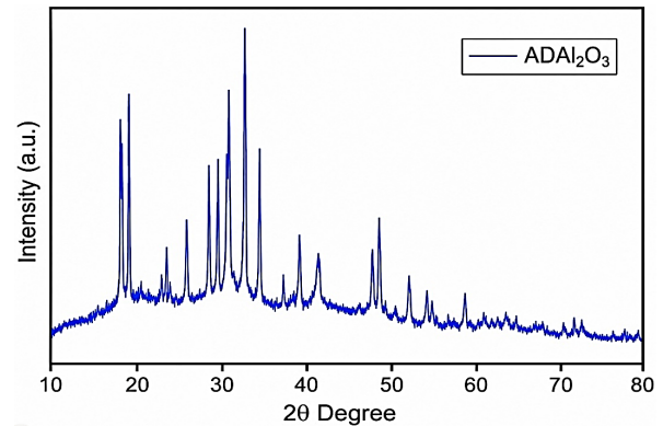
Figure 5. XRD analysis of \text{Al}_2\text{O}_3 nanoparticles
