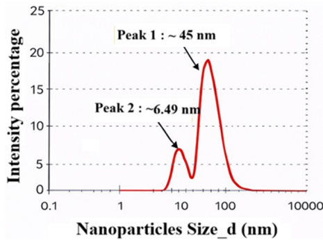
Figure 3. DLS analysis of \text{Al}_2\text{O}_3 nanodielectric
