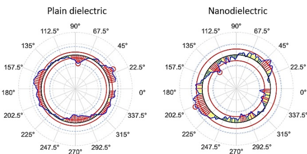
Figure 14. Polar plots for roundness: Inconel 718
