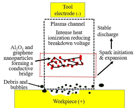
Figure 8. Material erosion in nanodielectric EDM
