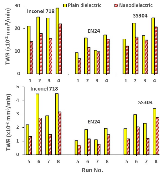
Figure 11. Tool wear rate varying with cutting conditions for different materials
