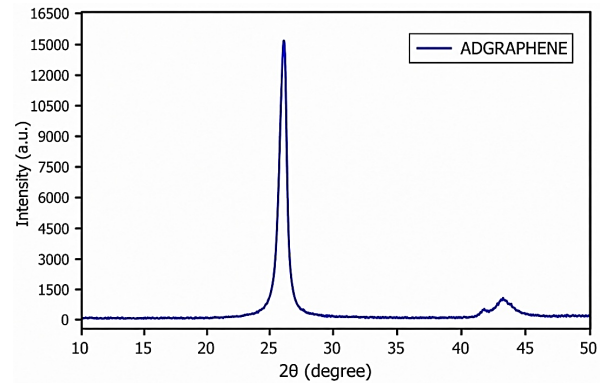
Figure 6. XRD analysis of Graphene nanoparticles
