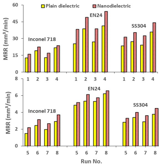
Figure 9. MRR varying with cutting conditions for different materials
