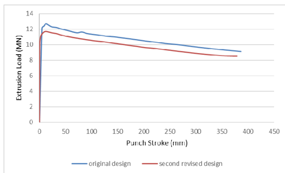
Figure 13. Comparison of the load values versus punch stroke
