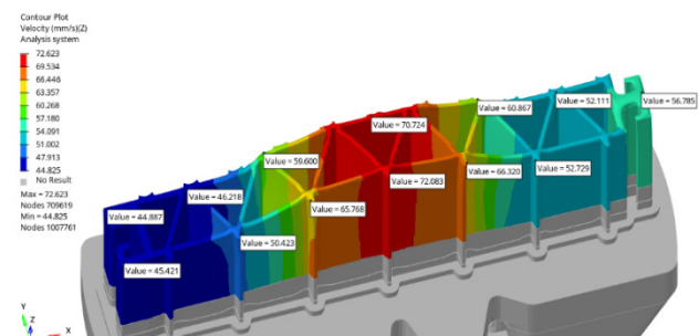
Figure 4. Exit velocity distribution of initial die design of the carrier panel
