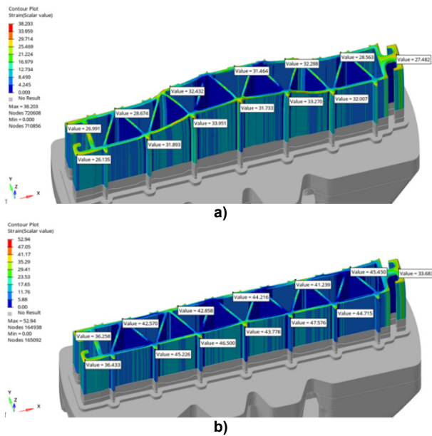
Figure 12. Strain distribution of carrier panel a) Initial design b) Second revised design
