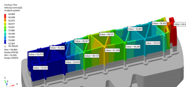
Figure 7. Exit velocity distribution of the revised die design of carrier panel
