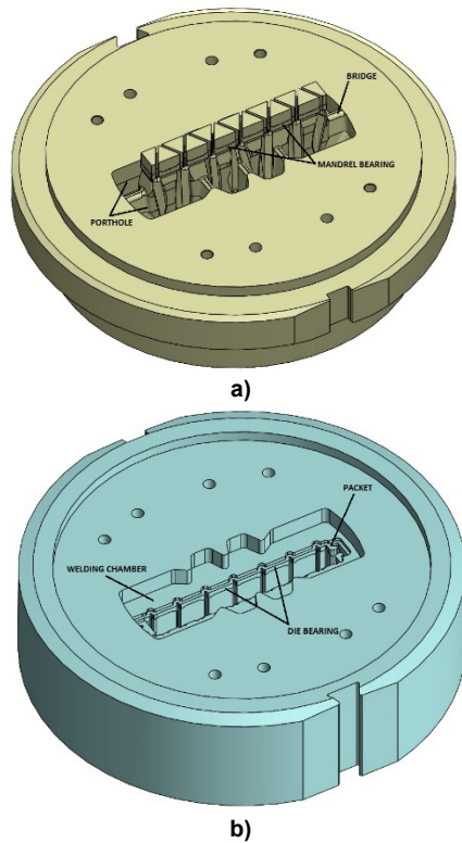
Figure 3. Example of disassembled porthole die of the carrier panel profile a) mandrel and b) die plate
