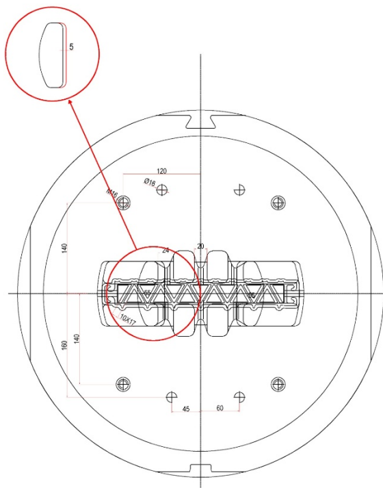
Figure 6. Revised design of the carrier panel profile die
