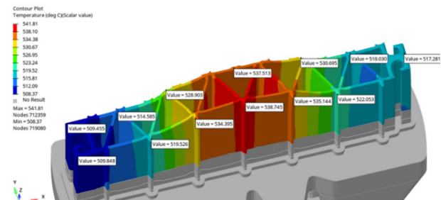
Figure 5. Exit temperature distribution of initial die design of the carrier panel
