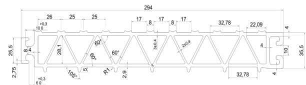
Figure 1. Geometry and dimensions of the profile
