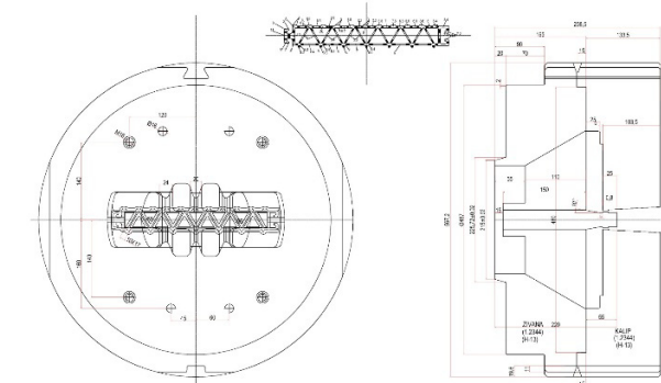
Figure 2. Initial design and dimensions of the carrier panel profile die
